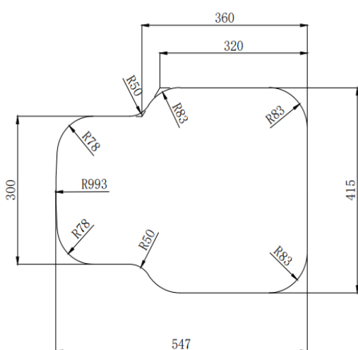
Undermount Installation
