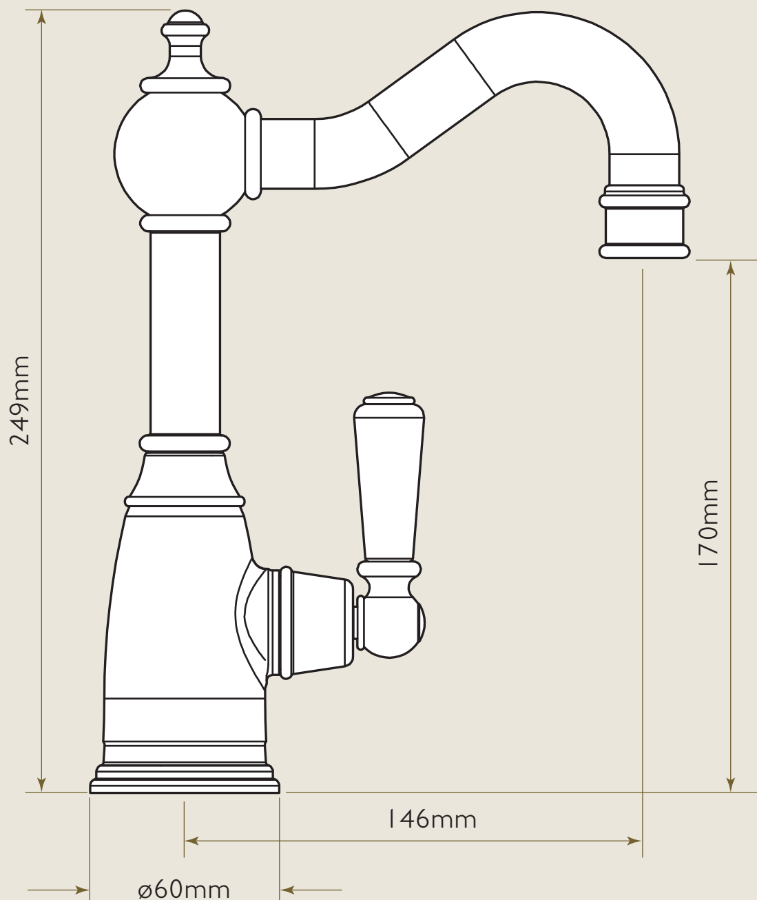
SINGLE LEVER WATER FILTER TAP
