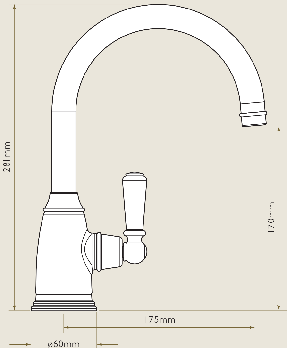
SINGLE LEVER WATER FILTER TAP
