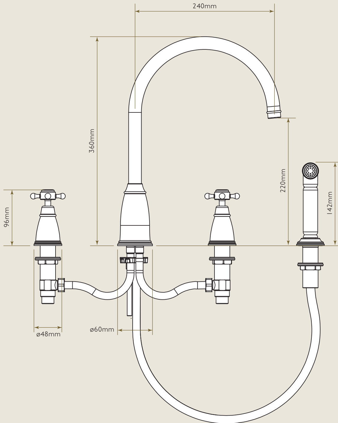
4 HOLE MIXER TAP WITH SIDE SPRAY AND CROSSHEAD HANDLES
