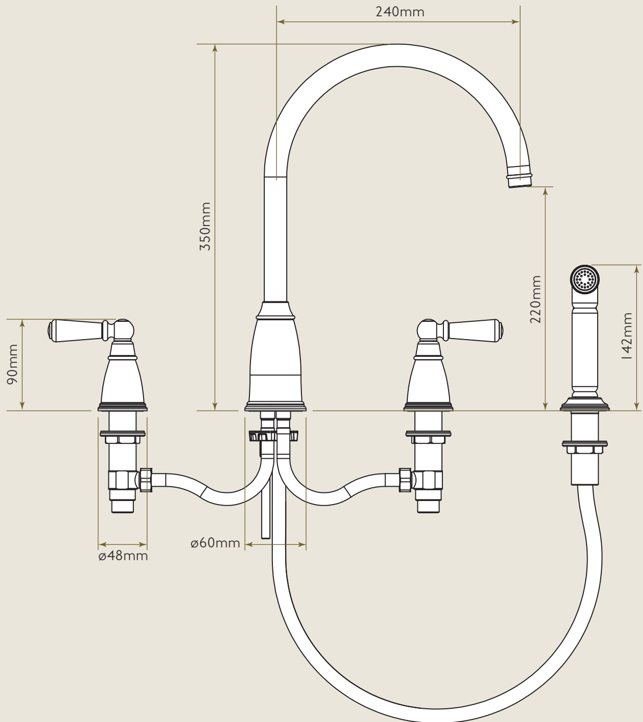
TWIN LEVER 4 HOLE MIXER TAP WITH SIDE SPRAY AND LEVER HANDLES
