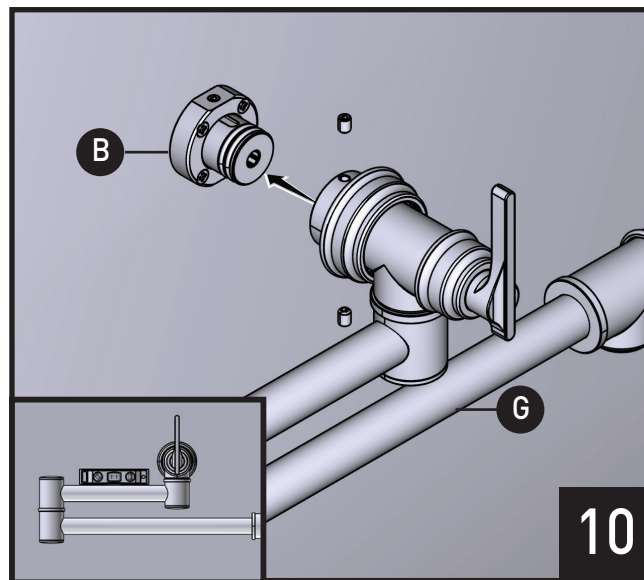
Install Tap Body (G) onto Wall Connector (B) and level it.
