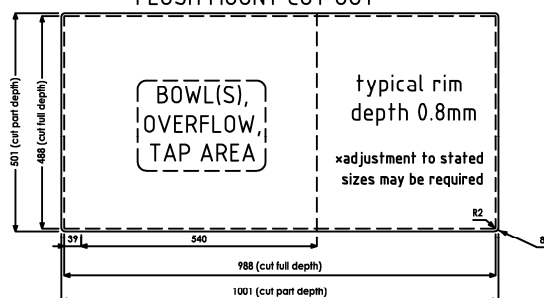
FLUSH MOUNT CUT OUT
