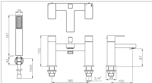
Fervour Bath shower mixer
